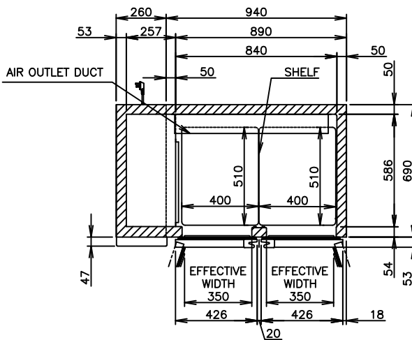
GN PAN STOCK AREA
