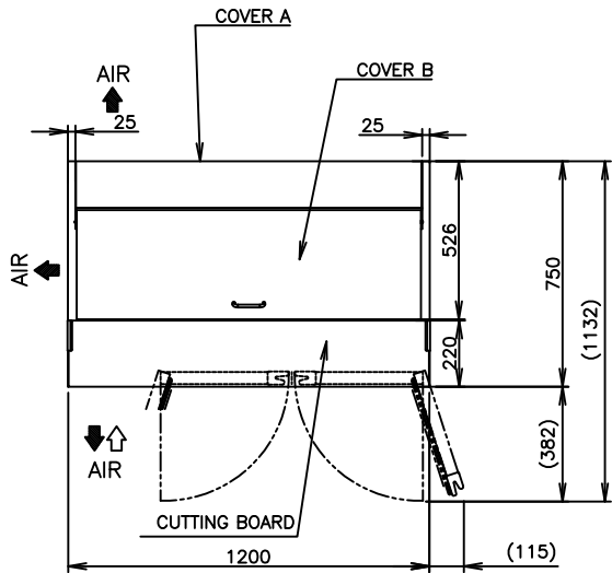
VIEW A
